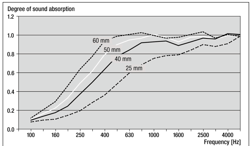
Diagram 4: Degree of sound absorption of Basotect G+ as a function of the thickness, according to DIN EN ISO 354 (reverberation room)
