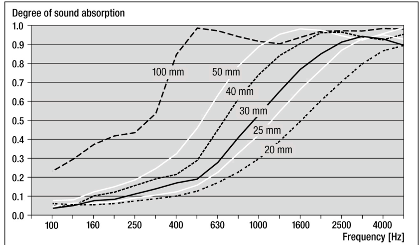
Diagram 3: Degree of sound absorption of Basotect® G+ as a function of the thickness, according to ISO 10534-2 (impedance tube).
