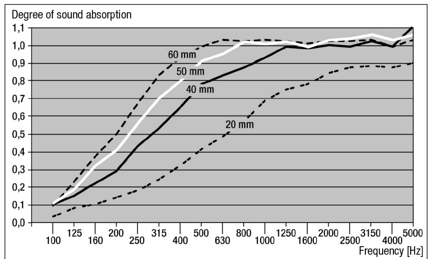
Diagram 2: Degree of sound absorption, \alpha_s , of Basotect® G depending on the thickness according to DIN EN ISO 354 (reverberation room)
